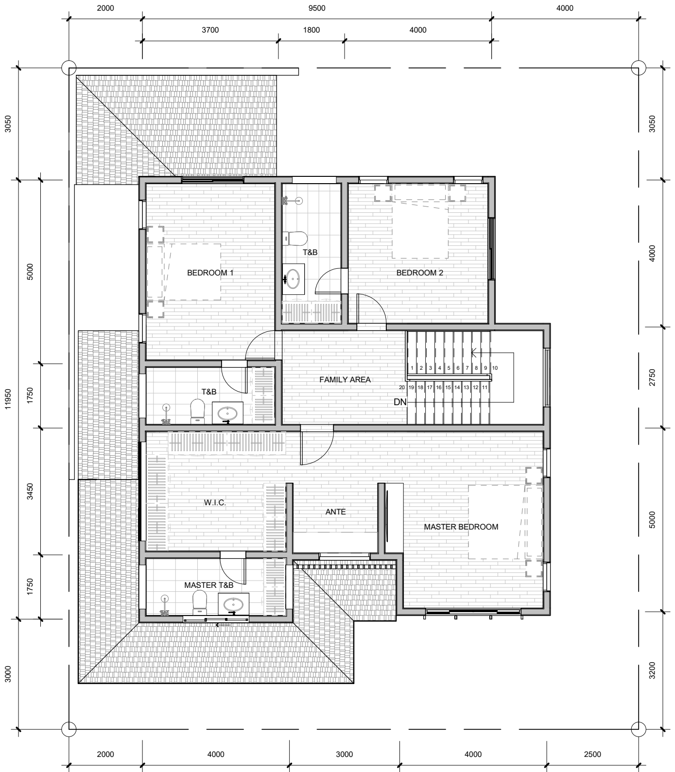
2 2ND FLOOR PLAN NOT TO SCALE
